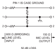
A15LA WIRING DIAGRAM
